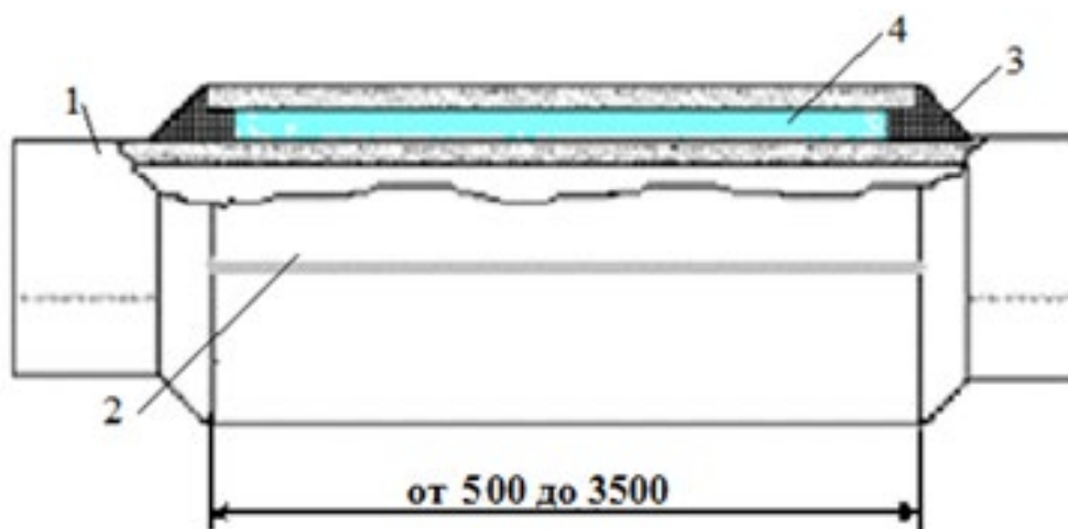
1 – pipeline; 2 – steel coupling; 3 – sealant; 4 – composite composition shape 1. Coupling type design P1, P1VD with CCT
